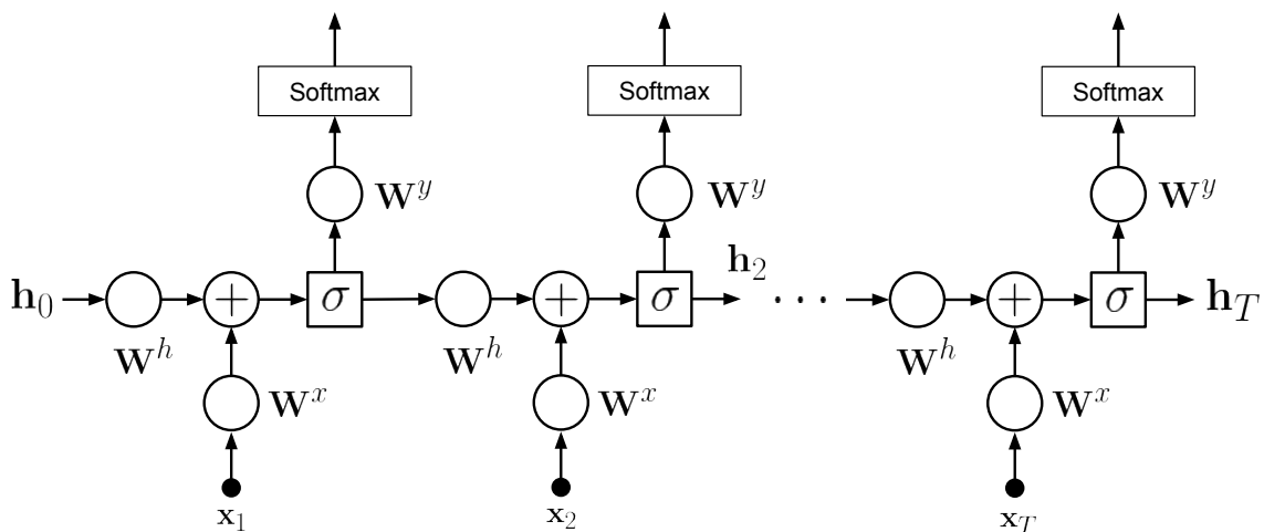
Figure 3.1: The simplest RNN can be seen as replicating a single hidden-layer FF network T times and passing the intermediate hidden variable \mathbf{h}_t across different steps. Note that all nodes operate over vector inputs e.g., \mathbf{x}_t \in \mathbb{R}^I . Circles indicate matrix multiplications.
