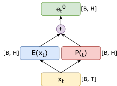
Figure 4.4: Construction of the input of the t -th token in layer e^0
