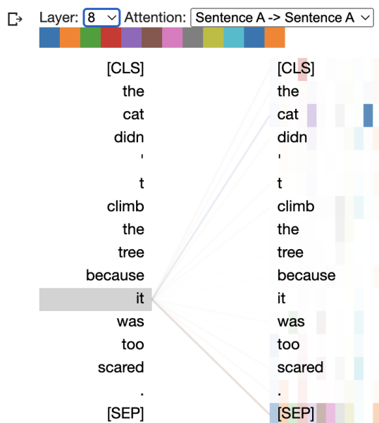
Figure 4.2: Self-Attention of the sample
